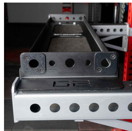
5/8" and 1" Holes
