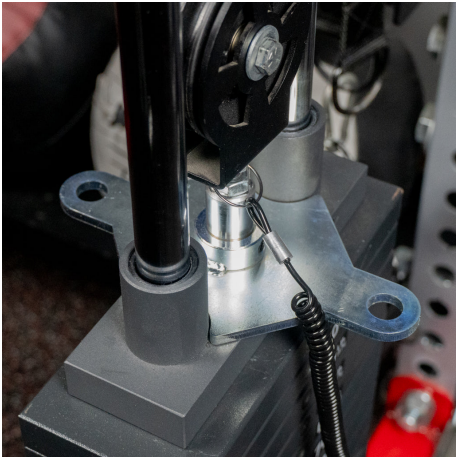
Top Plate
