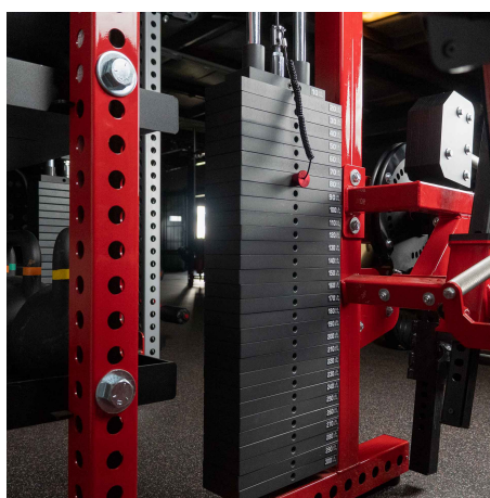
300 LBS 1:1 Ratio Stack
