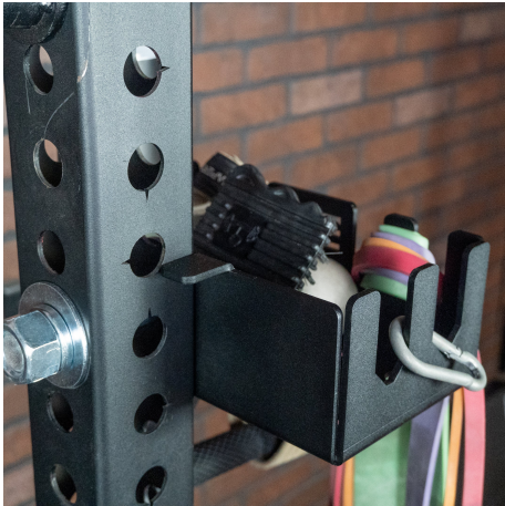
Anti-Rotation Tabs
