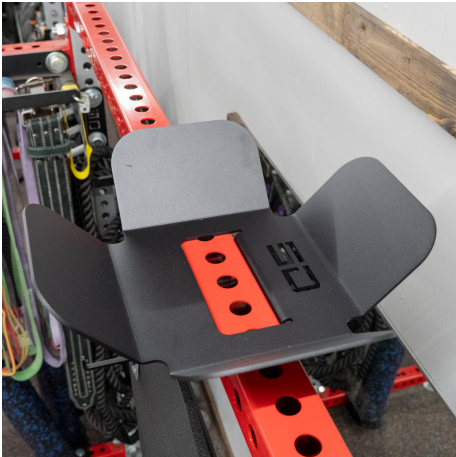
Bolt to 3x3" Tubing with 1" Holes
