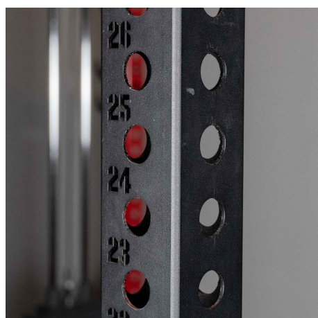
3x3" Tubing with Inline 1" Holes
