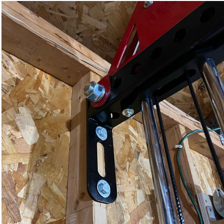
Mount To Garage Wall
