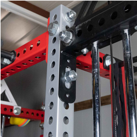
Mount to any 1" Hole Rack
