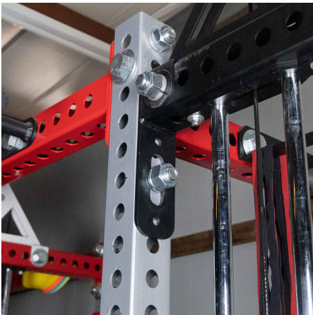
Mount to any 1" Hole Rack
