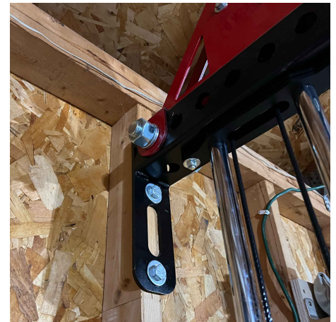
Mount To Garage Wall
