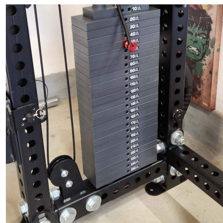
Add to 20" or 30" Crossmembers
