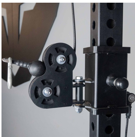
Pull Pin Adjustment
