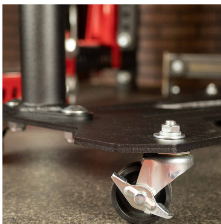
1/4" Steel Plate
