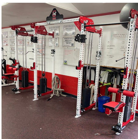
2 Lifting Stations no Trays
