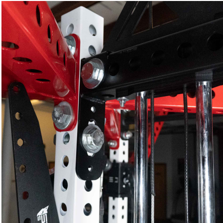
Slotted Crossmember
